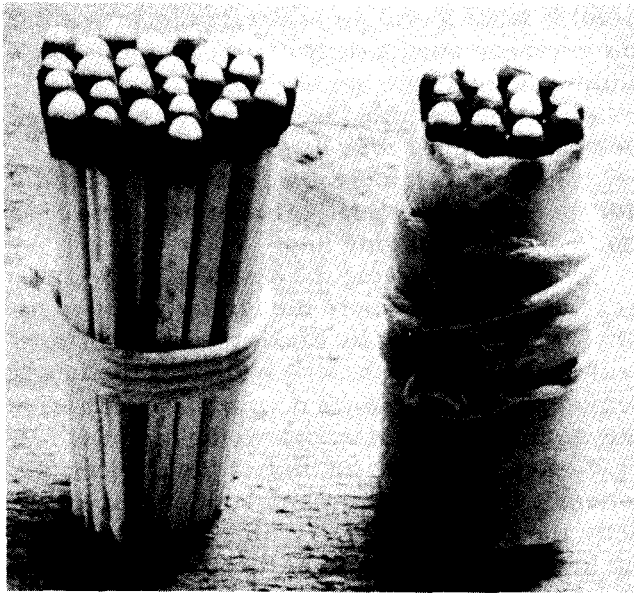
Two big matches, dipped, cooled, and with their strings trimmed. The one on the left will make a bigger initial fire because it has more matches; the one on the right will burn longer because it is surrounded by paper-soaked paraffin.
