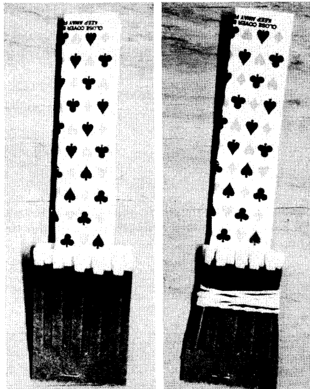
(Left) Turn the striker ninety degrees, so that it is parallel to the match sticks. Make sure it is centered. (Right) Wrap a rubber band around the match sticks, being careful to keep the striker perfectly centered. Getting the right amount of tension takes a little practice. If a rubber band is unavailable, the same thing can be done with tape or string, though not quite as easily.
