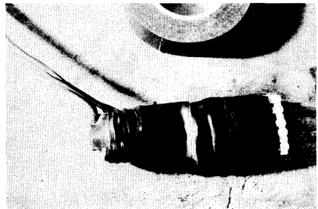
Add more match books and tape until the filament, the wire that holds it, and the base are completely covered. Make sure that at least one row of match heads is exposed and the top is open; fire will blow out the end.
