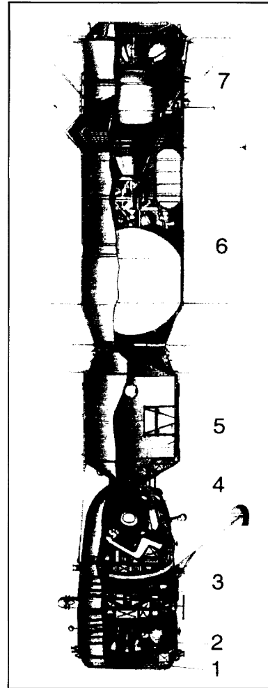
The 7K-9K-11K piloted circumlunar complex emerged in 1963 as a successor to the Vostok 7/11 conception. The image here shows the 7K spacecraft docked to the 9K translunar injection stage, which has been loaded with propellant by means of several 11K orbital tankers. The legend is (1) and (7) jettisonable compartments; (2) 7K aggregate compartment; (3) 7K instrument compartment; (4) 7K descent apparatus; (5) 7K living compartment; and (6) 9K rocket block. Note the close resemblance of the 7K to the future Soyuz spacecraft (reproduced from M. V. Keldysh, ed. Tvorcheskoye naslediye Akademika Sergeya Pavlovicha Koroleva izbrannyye trudy i dokumenty (Moscow: Nauka, 1980).)
