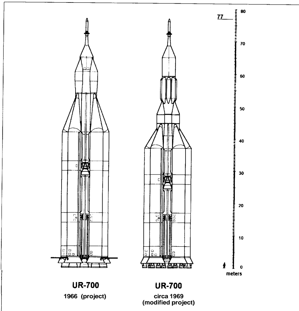
Shown are two variants of Chelomey's UR 700 booster from 1966 and circa 1969 (copyright Peter Corin)
