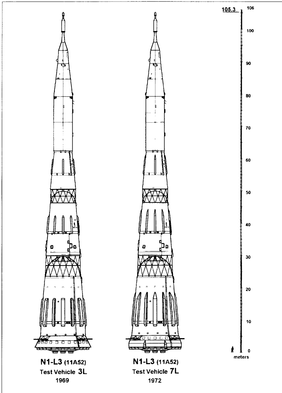
On the left is the early test variant of the N1 rocket as originally conceived in the mid-1960s. On the right is a slightly modified version designed in the early 1970s. The main external differences were in the fairing at the bottom of the first stage and the length of the vertical conduits on the first and second stages. (copyright Peter Corin)
