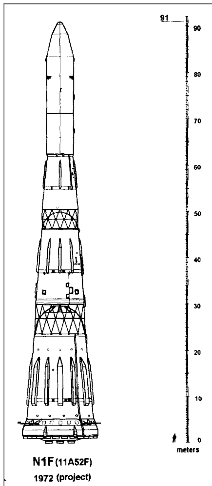
The NIF variant of the basic N1 rocket was intended to launch the advanced L3M complex for long-duration stays on the Moon. The program received preliminary approval by the Council of Chief Designers in May 1972 (copyright Peter Gorin)
