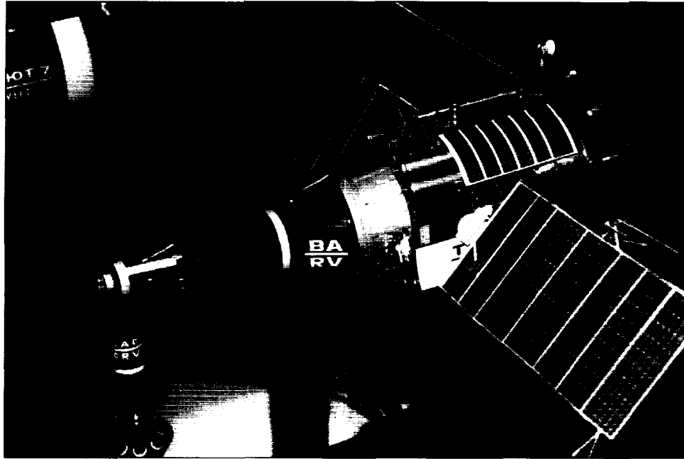
Here is a model of Vladimir Chelomey's Transport Supply Ship (TKS) which was meant to be part of the Almaz military space station complex. The conical segment at the left is the reentry capsule, apparently patterned after the US Air Force's Gemini B spacecraft. The vertically placed component at the left is the launch escape system. (copyright Dietrich Haeseler)
