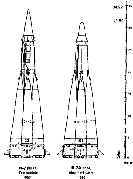
The Soviet R 7 ICBM The left diagram is the original variant of the missile the 8K71 as it was flown in 1957 The later operational version the R 7A or 8K74, is shown on the right (copyright Peter Gorin)
