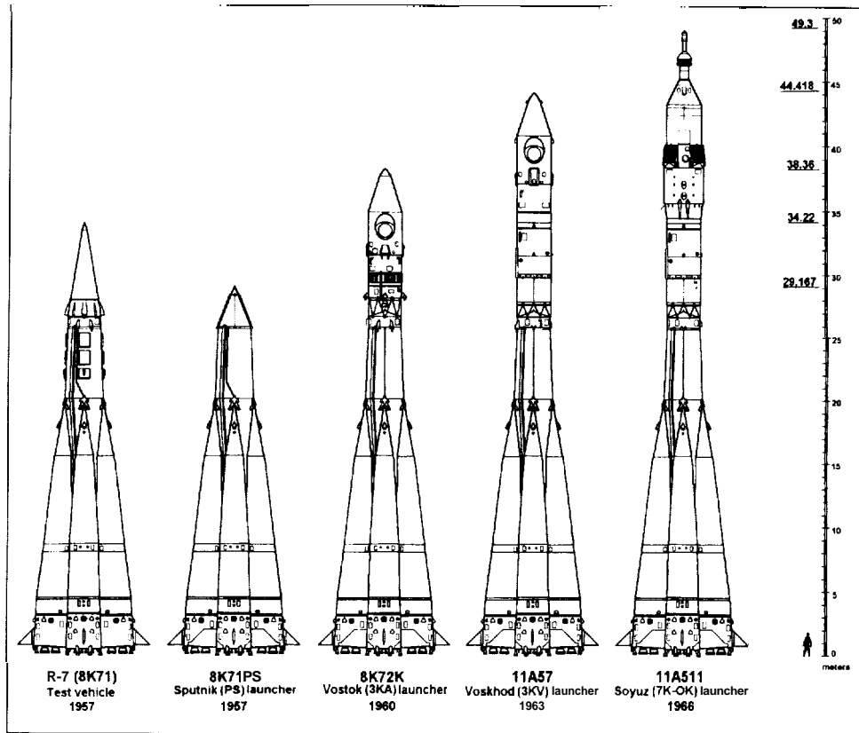
This shows the evolution of Soviet space launch vehicles in the early years. From the left are the R 7 ICBM, the Sputnik launcher, the Vostok launcher, the Voskhod launcher, and the Soyuz launcher (copyright Peter Gorin)
