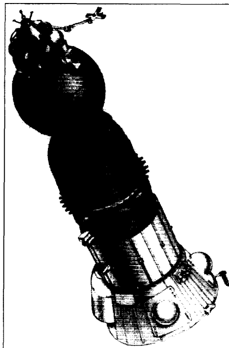
The Lunar Orbital Ship (LOK) of the Soviet L3 lunar landing complex would play an analogous role to the Apollo Command-Service Module remaining in lunar orbit while the lander carried a single cosmonaut to the surface of the Moon. Note the skirt at the base of the spacecraft, a visible difference from the basic Earth orbital Soyuz. (copyright VideoCosmos Co. via Dennis Newkirk)
