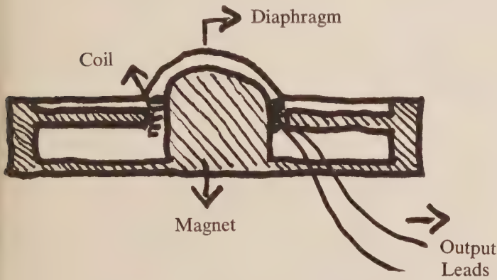
Figure 15. Dynamic Microphone.
