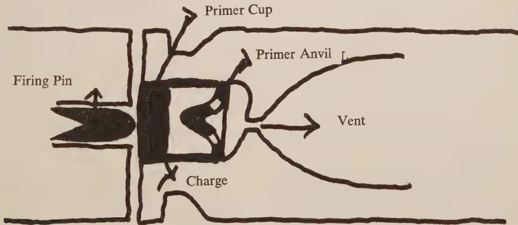
Figure 40. Boxer primer.
