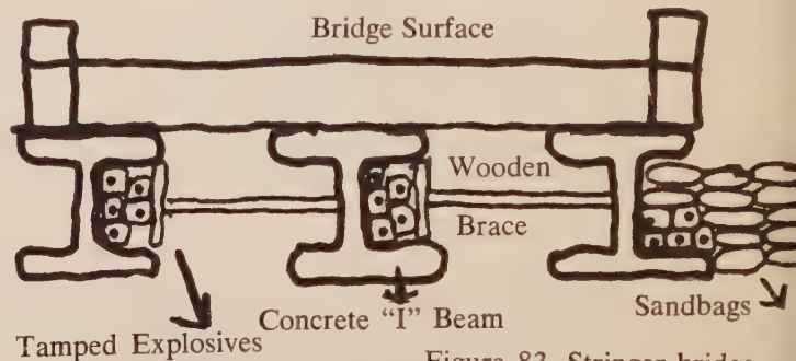
Figure 83. Stringer bridge.
