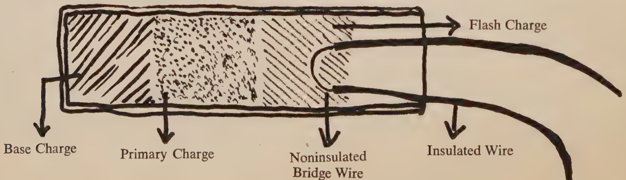
Figure 75. Electrical blasting cap.
