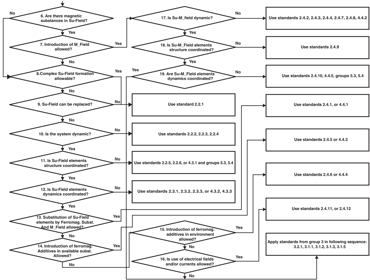
FIGURE 15.1 Algorithm for use of standards.
