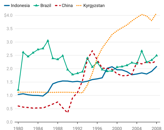
Fig. 1. Cost of meeting basic needs (2011 PPP$), 1980–2008. Based on Moatsos (2021).
