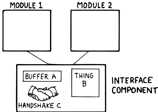
Figure 3.9: Use of the interface component.
