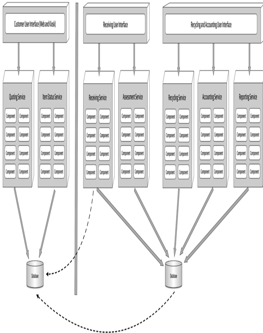
Figure 13-8. Electronics recycling example using service-based architecture
