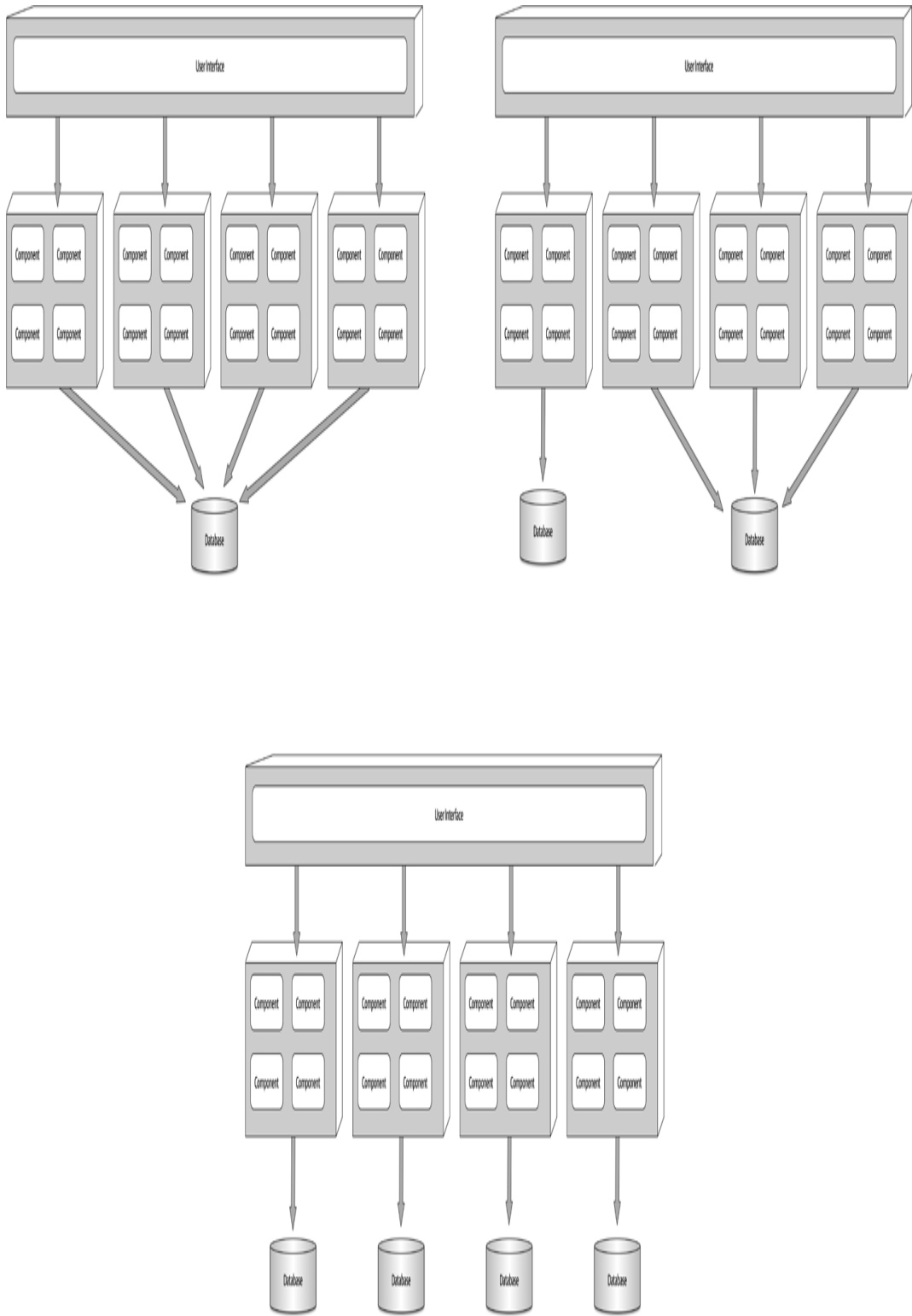
Figure 13-3. Database variants
