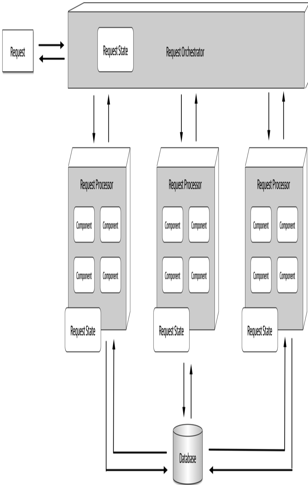
Figure 14-1. Request-based model
