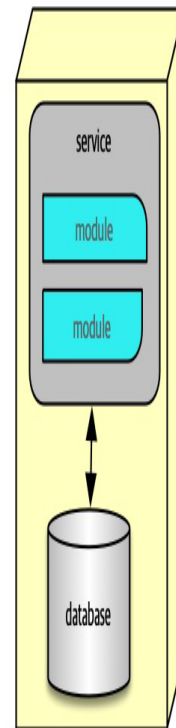
Distributed service
