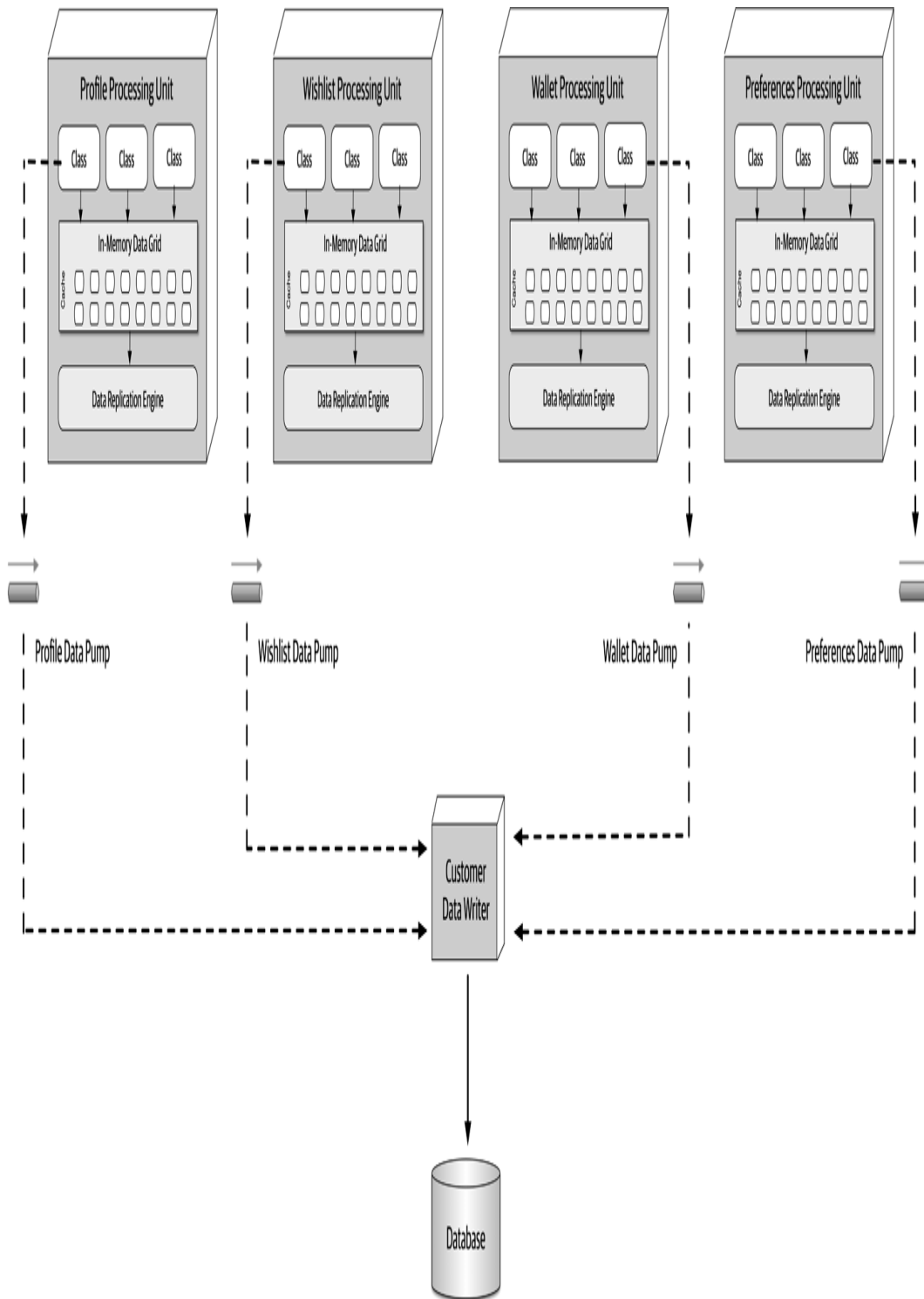
Figure 15-8. Domain-based data writer
