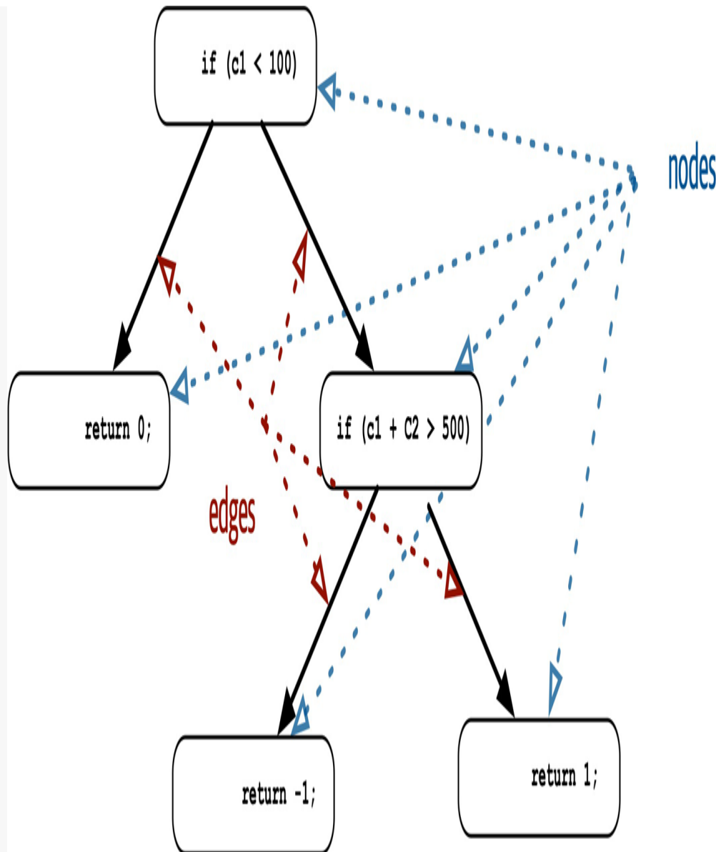
Figure 6-1. Cyclomatic Complexity for the decision function
