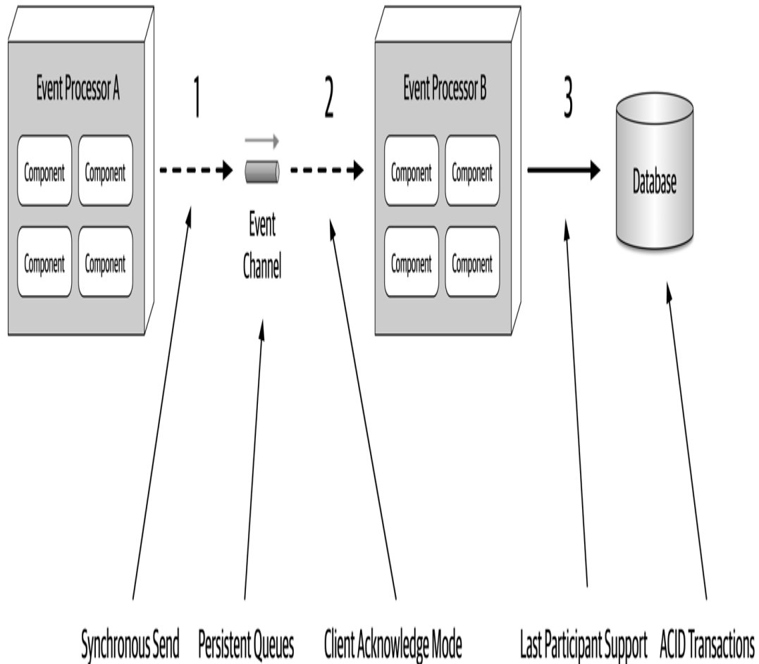
Figure 14-17. Preventing data loss within an event-driven architecture
