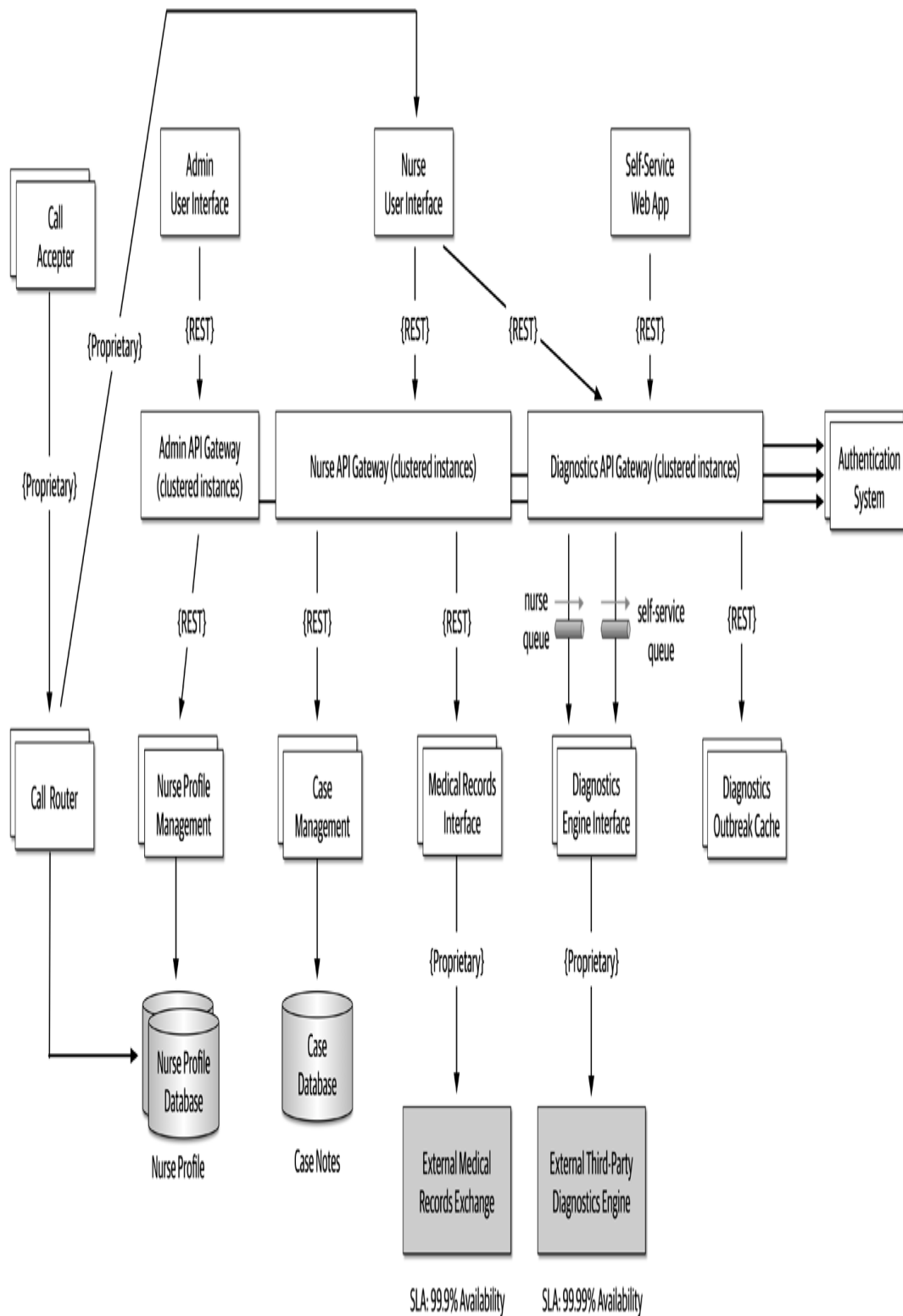
Figure 20-13. Final architecture modifications to address security risk
