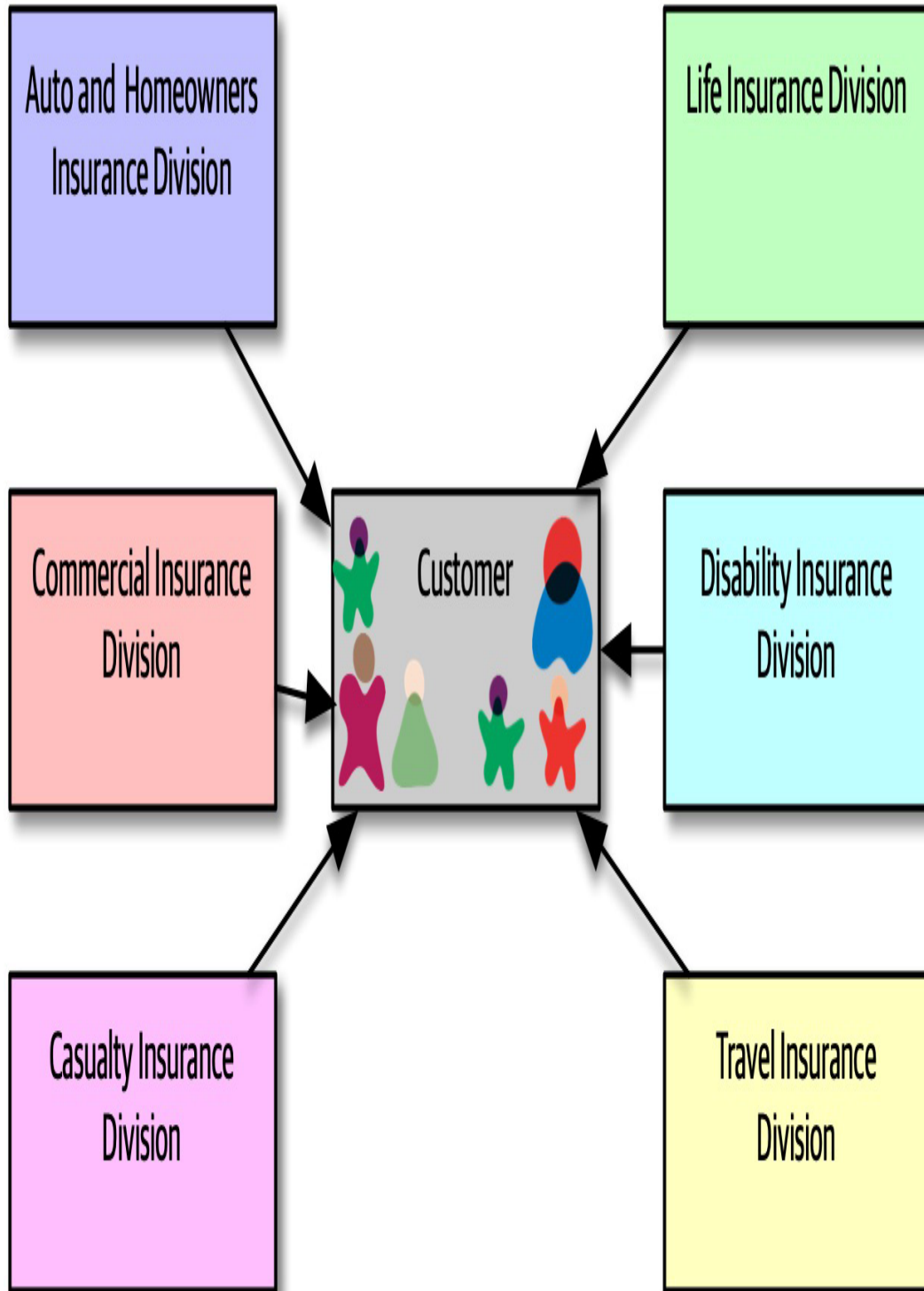
Figure 16-4. Building canonical representations in service-oriented architecture
