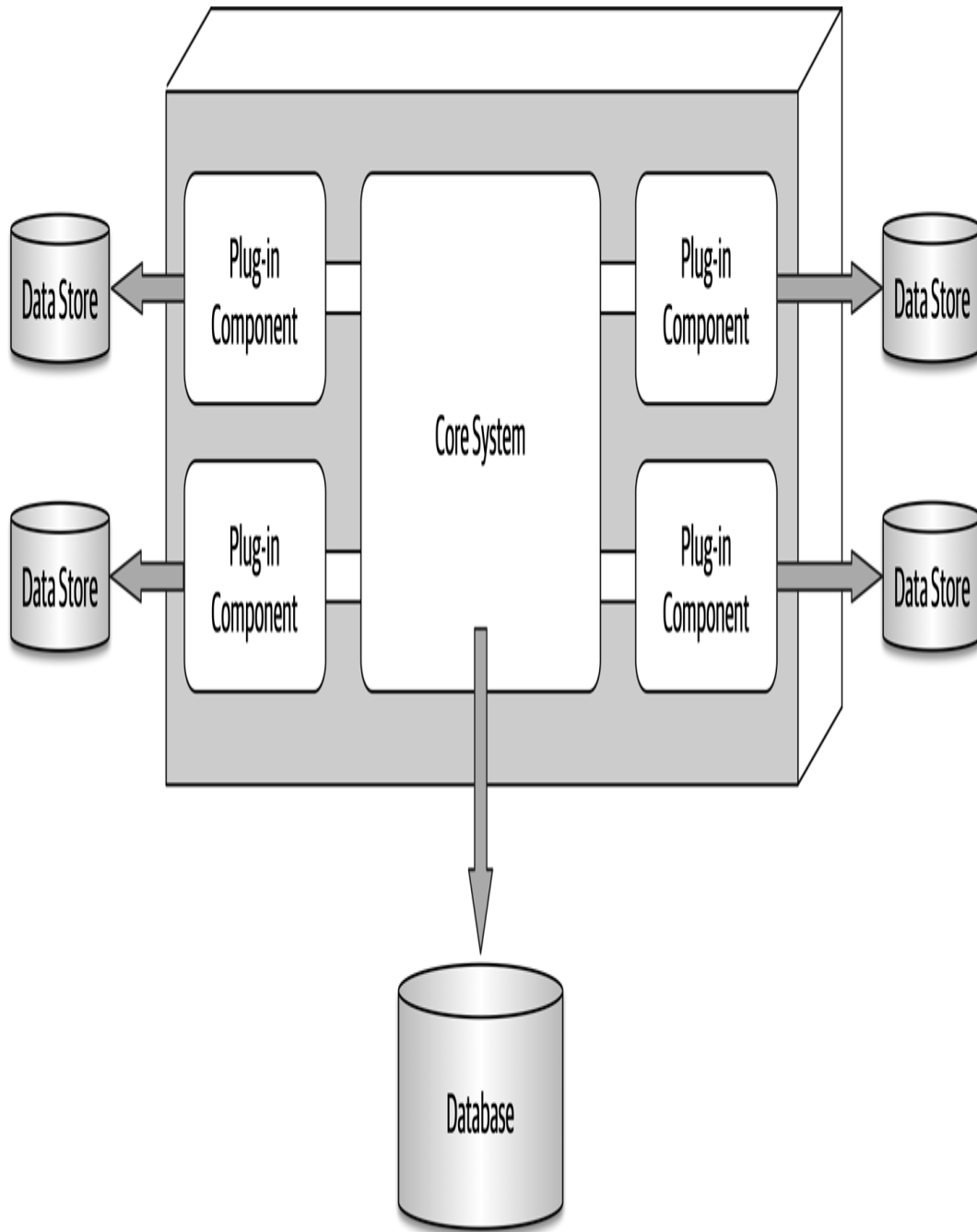
Figure 12-7. Plug-in components can own their own data store
