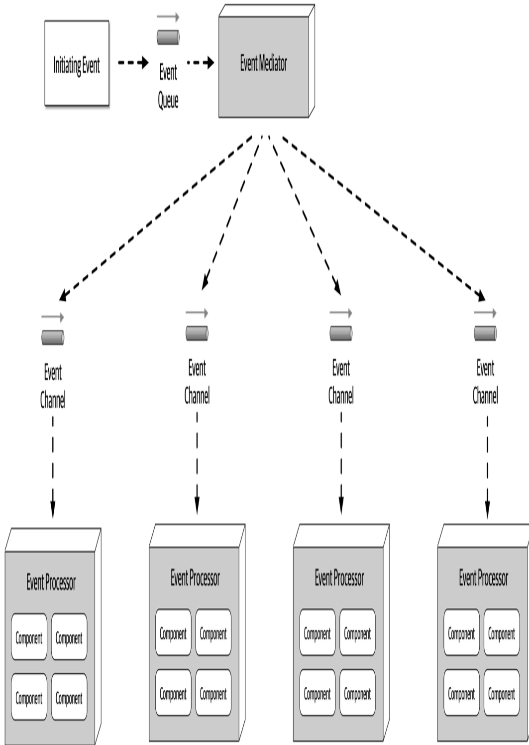
Figure 14-5. Mediator topology
