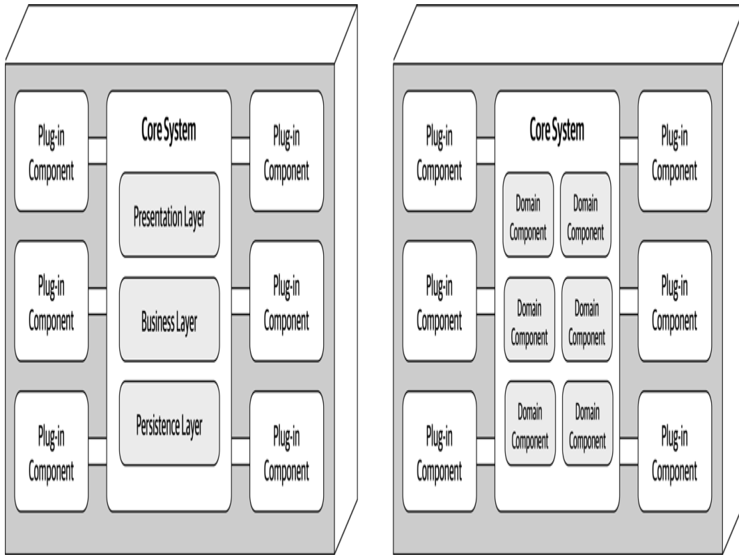
Layered Core System (Technically Partitioned)
