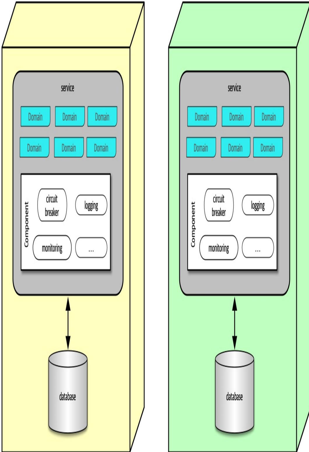
Figure 17-2. The sidecar pattern in microservices
