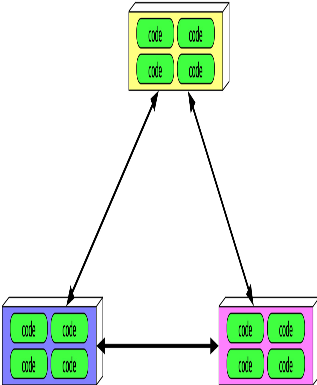
Figure 6-3. Cyclic dependencies between components
