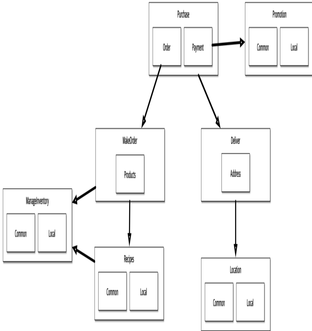
Figure 8-6. A domain-partitioned design for Silicon Sandwiches
