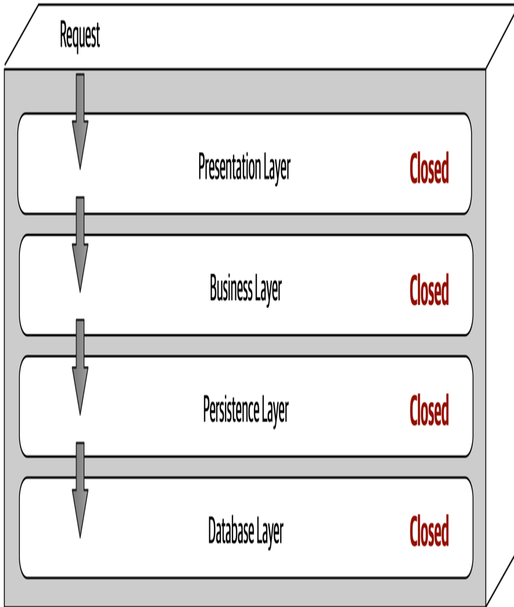
Figure 10-3. Closed layers within the layered architecture
