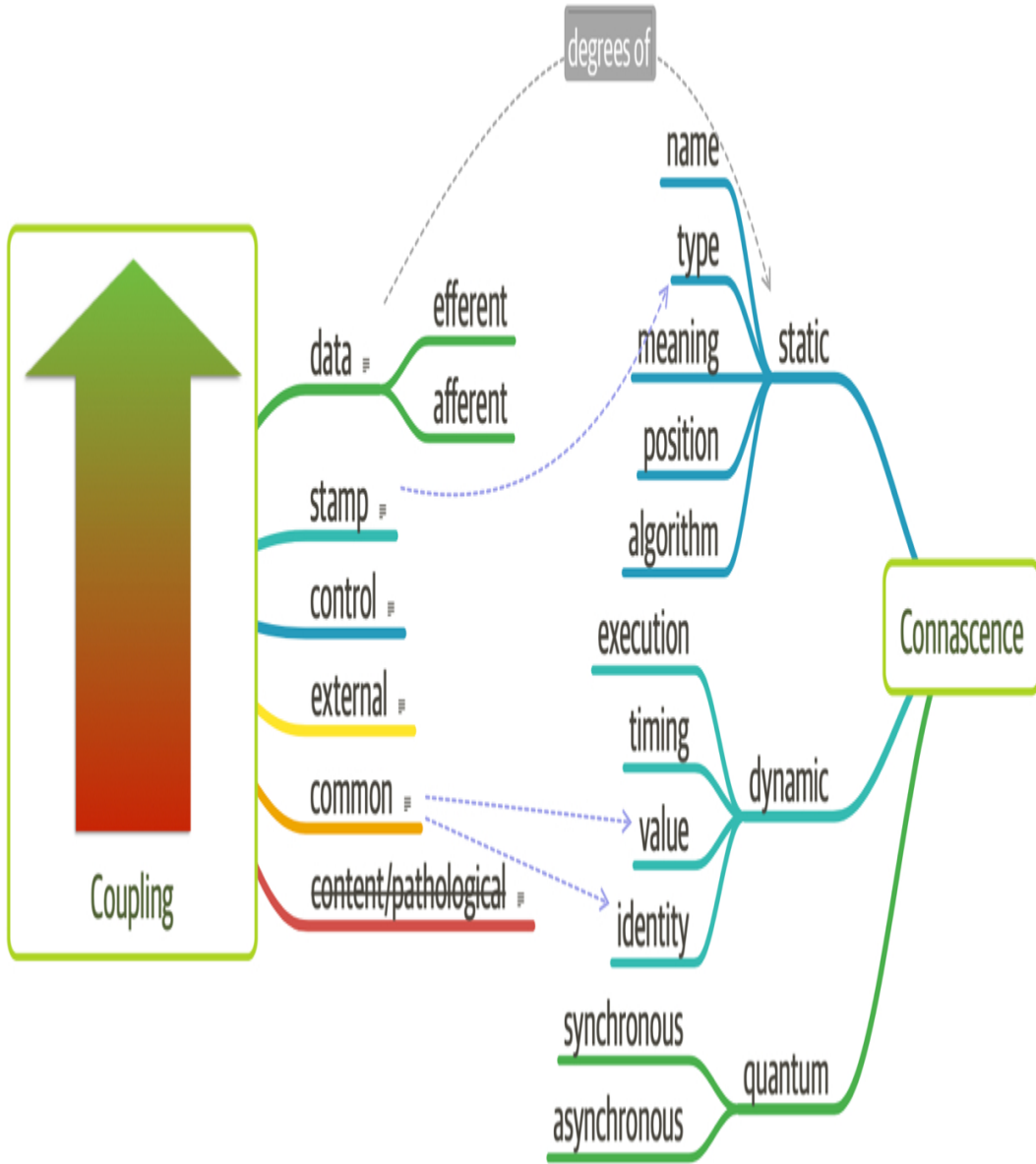
Figure 7-1. Adding quantum connascence to the unified diagram
