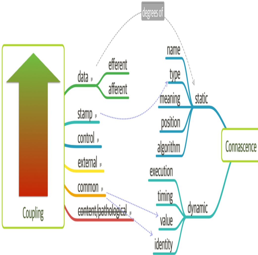
Figure 3-6. Unifying coupling and connascence
