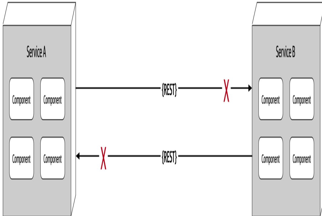
Figure 9-2. The network is not reliable
