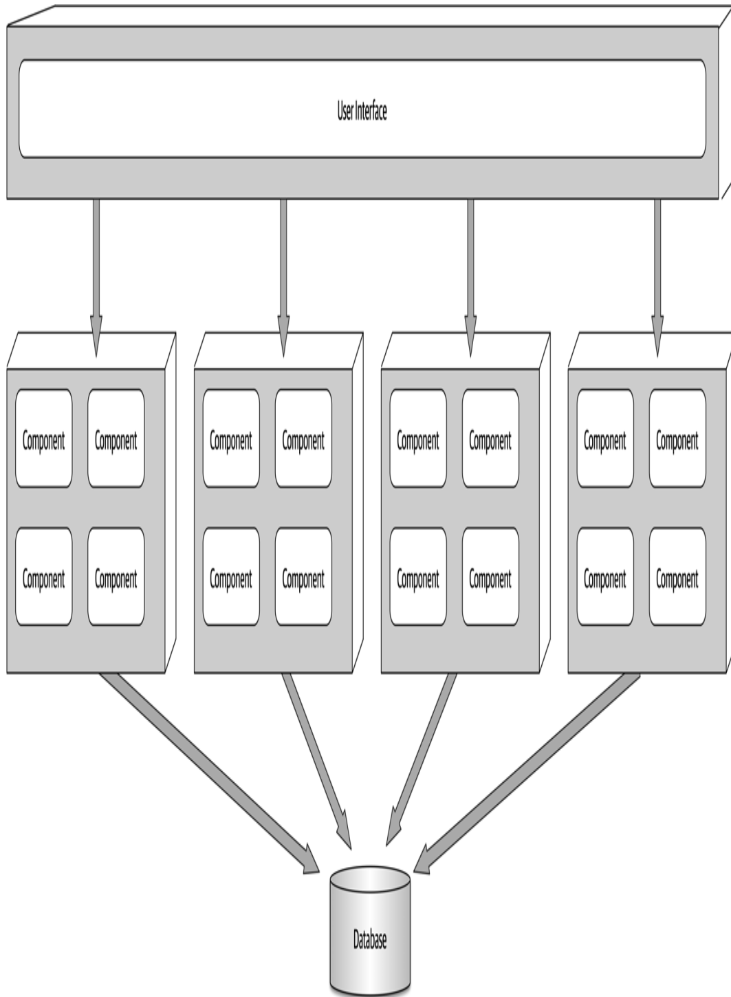
Figure 13-1. Basic topology of the service-based architecture style
