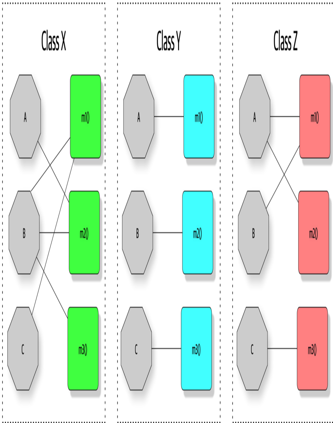
Figure 3-1. Illustration of the LCOM metric, where fields are octagons and methods are squares
